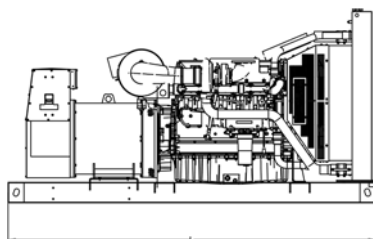
Open: (inches) 139L x 47W x 78H Weight (lbs.) 10,150
