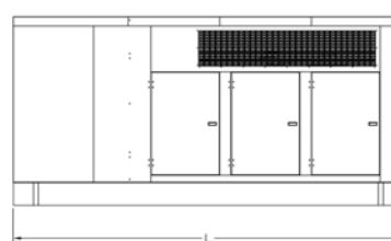
Deluxe: (inches) 188L x 64W x 89H Weight (lbs.) 13,200
