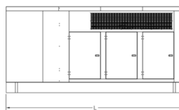
Deluxe: (inches) 188L x 64W x 82H Weight (lbs.) 13,200
