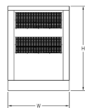
Deluxe: (inches) 188L x 64W x 82H Weight (lbs.) 13,200
